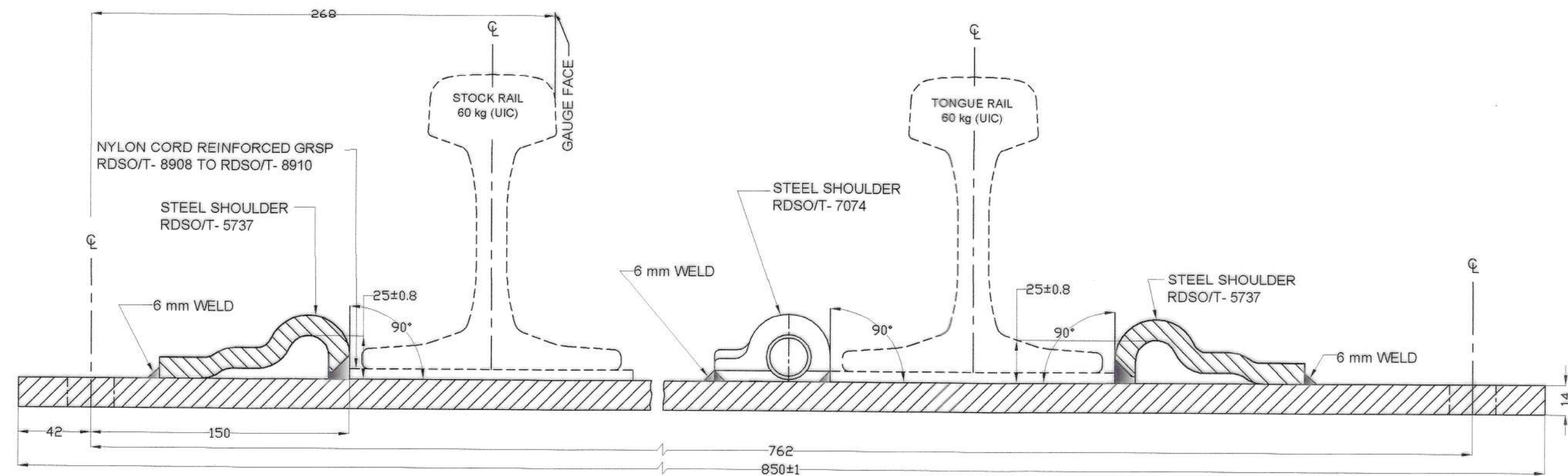
SECTIONAL ELEVATION ON AB
