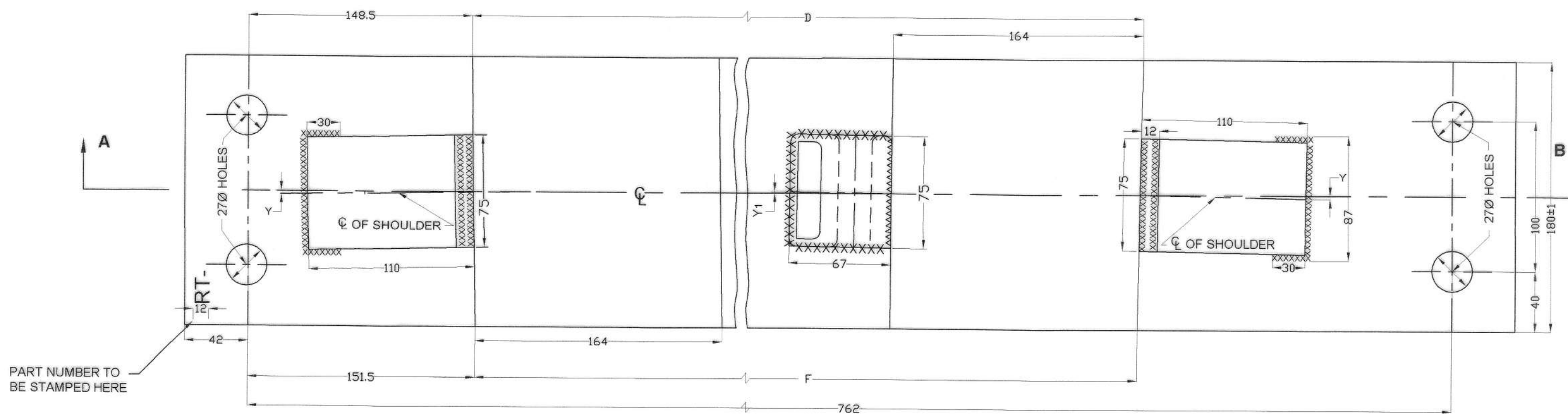
SECTIONAL ELEVATION ON AB
